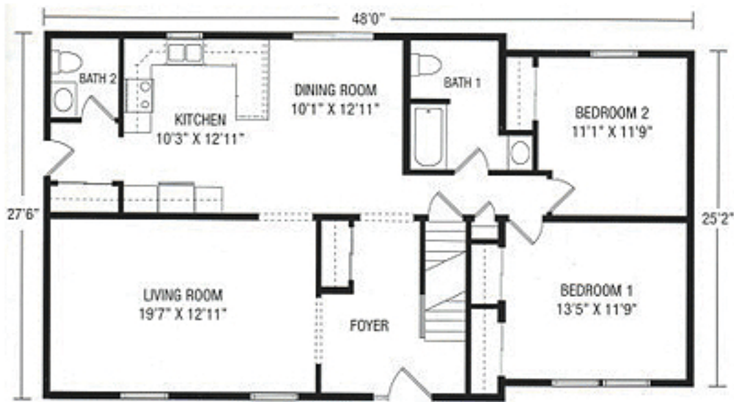
first floor
